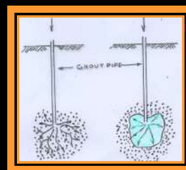
Permeation Compaction
