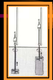
Jet Grouting
